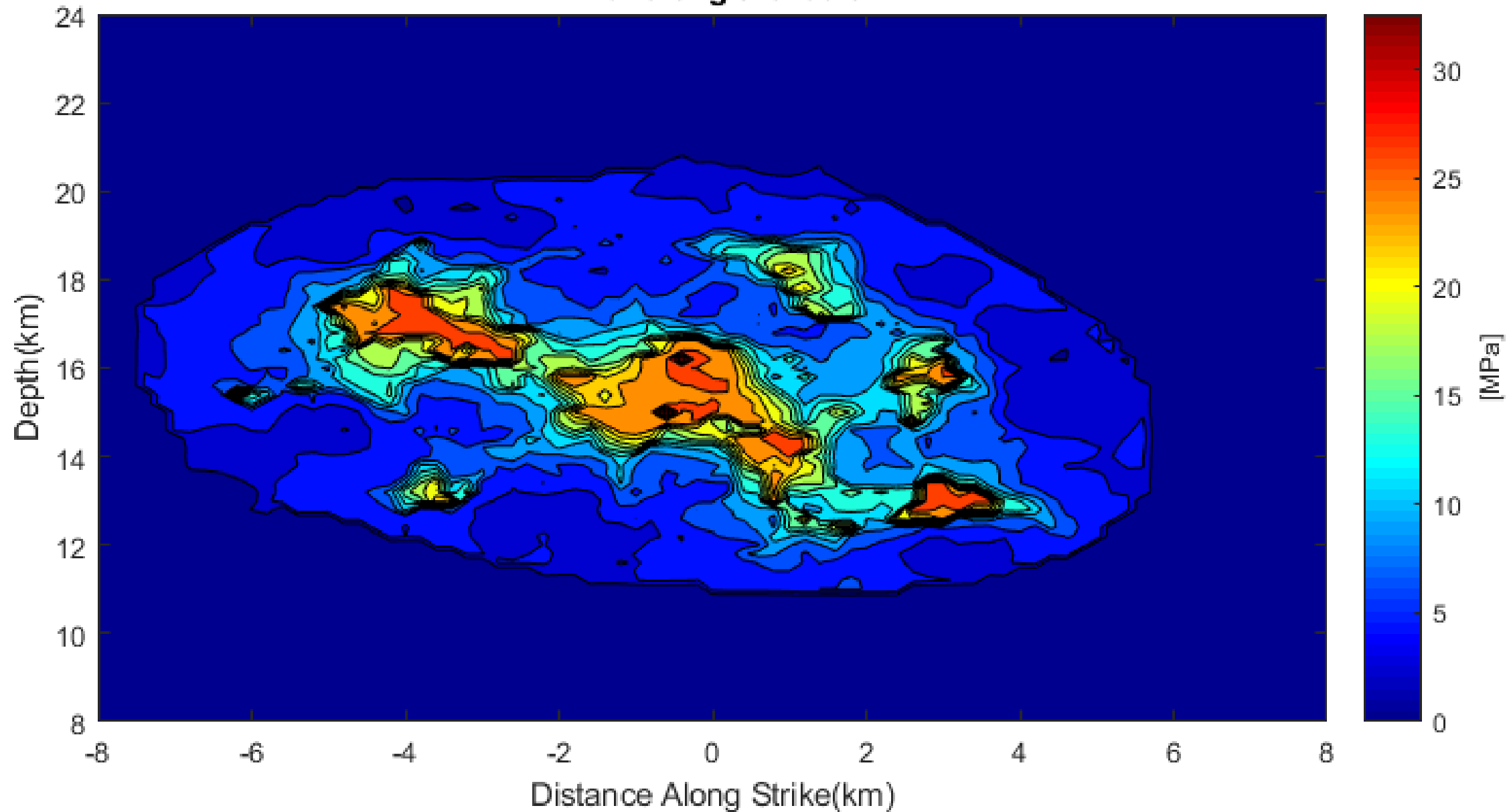
\Delta \sigma along the fault
